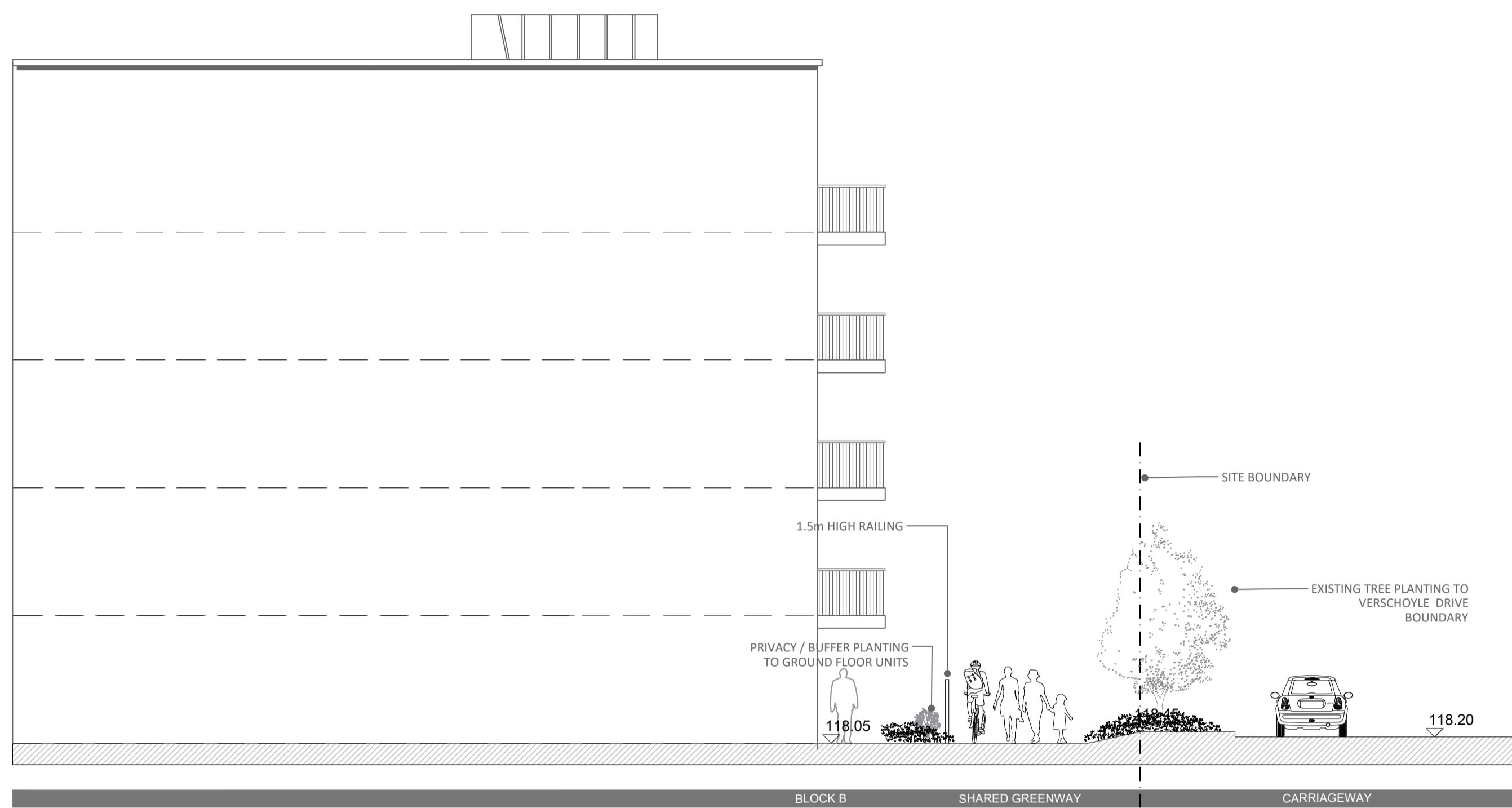
SECTION C-C
